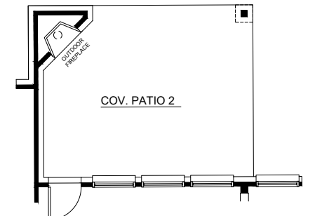
OPTIONAL OUTDOOR FIREPLACE AT COVERED PATIO 2
