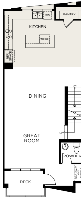
SECOND FLOOR
