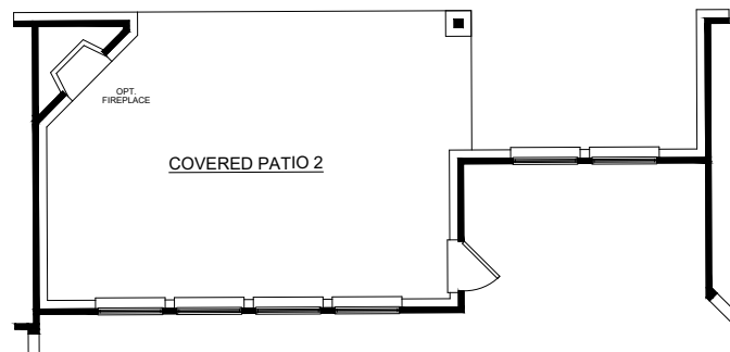
OPTIONAL COVERED PATIO 2 W/ OPTIONAL OUTDOOR FIREPLACE
