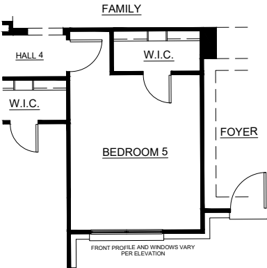
OPTIONAL BEDROOM 5 ILO DINING ROOM
