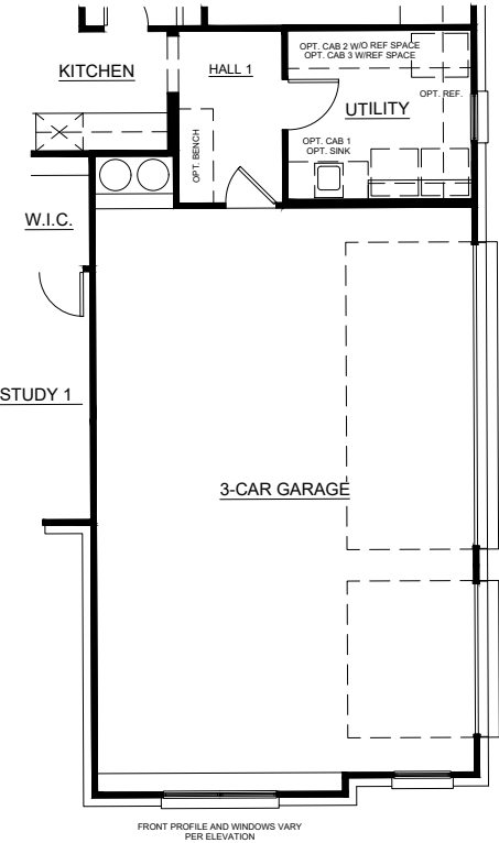
OPTIONAL 3-CAR GARAGE
