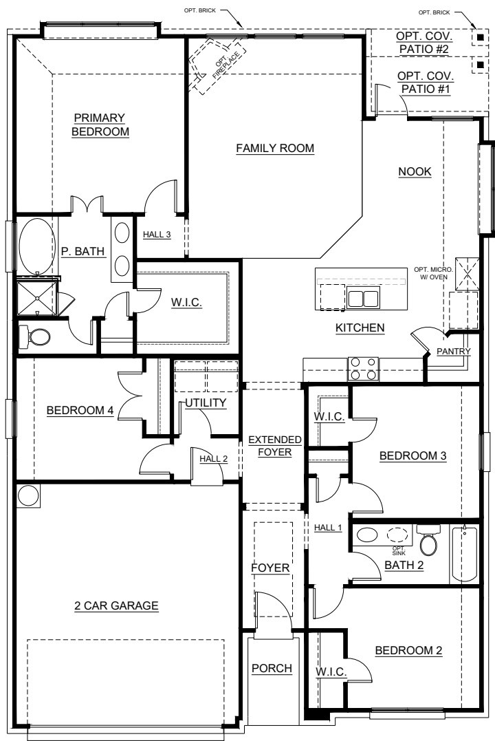
FIRST FLOOR
