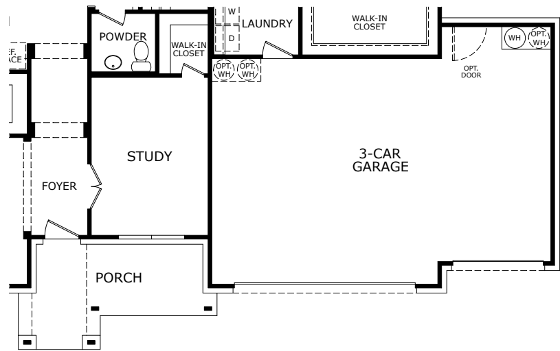
OPTIONAL 3-CAR GARAGE
