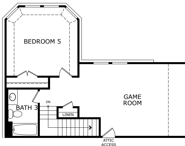
OPTIONAL SECOND-FLOOR BEDROOM 5 W/ GAME ROOM AND BATH 3
