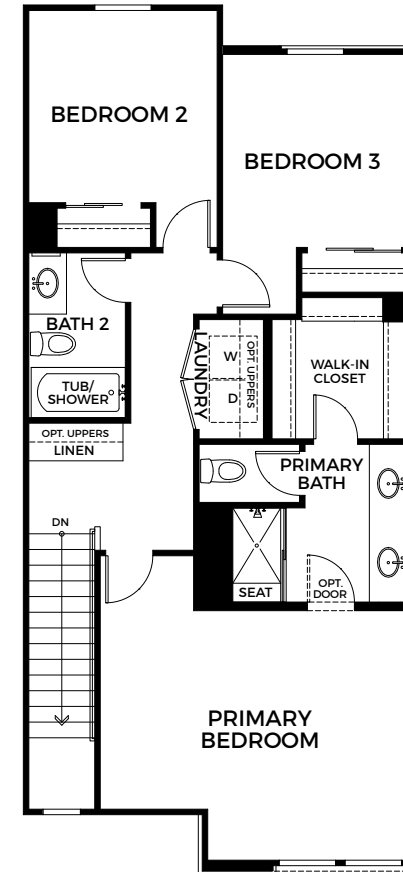
Third Floor
