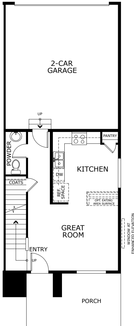
FIRST FLOOR
