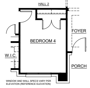
OPTIONAL BEDROOM 4 ILO FLEX ROOM
