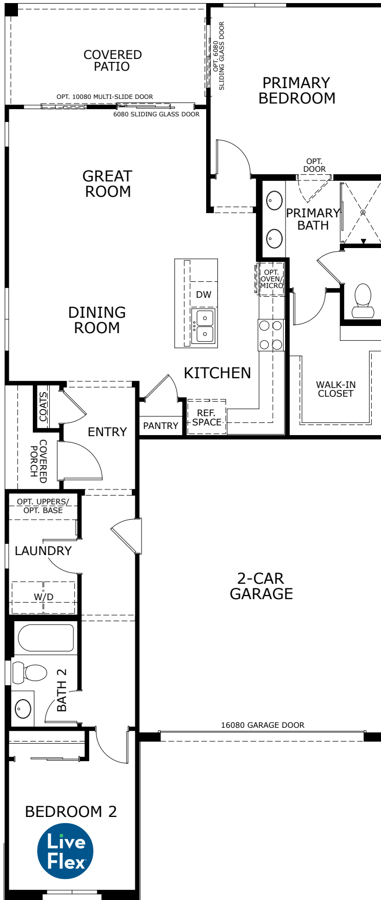
FLOOR PLAN
