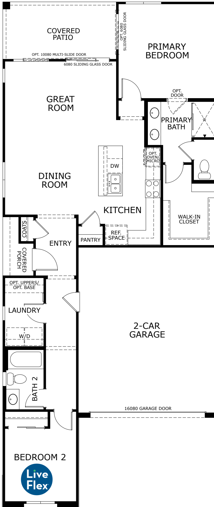
FLOOR PLAN
