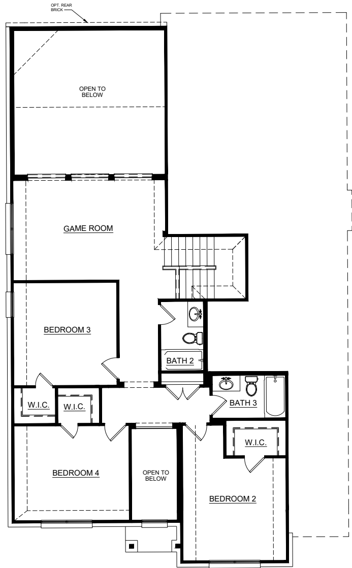
SECOND FLOOR
