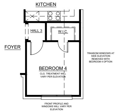
OPTIONAL BEDROOM 4 I/O DINING ROOM
