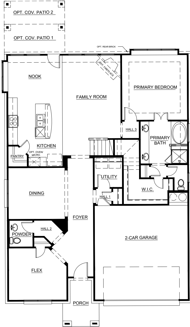
FIRST FLOOR
