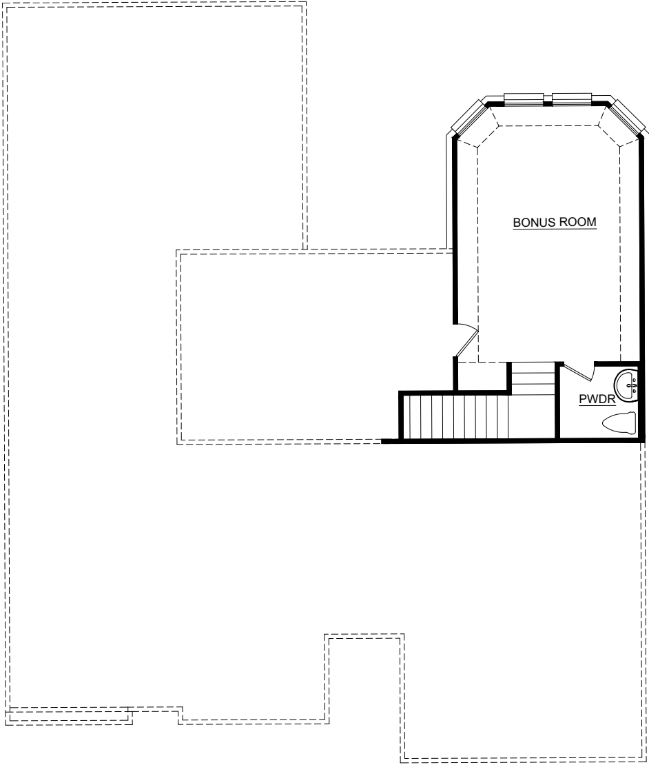
SECOND FLOOR
