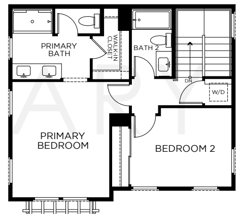
THIRD FLOOR
