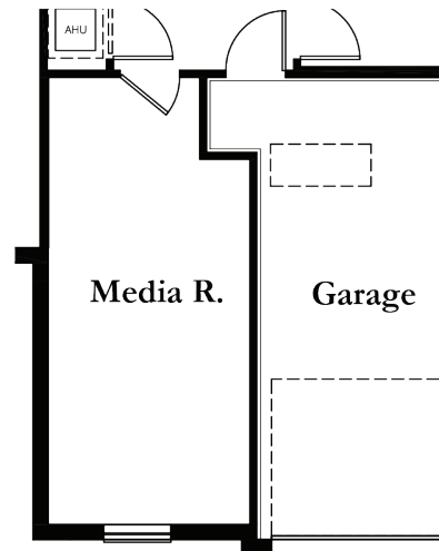
OPTIONAL MEDIA ROOM I.L.O. 3RD CAR *ADDS 193 LIVING SQ. FT.
