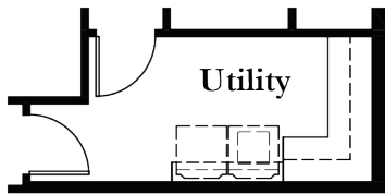
OPTIONAL DELUXE UTILITY ROOM *ADDS UPPERS
