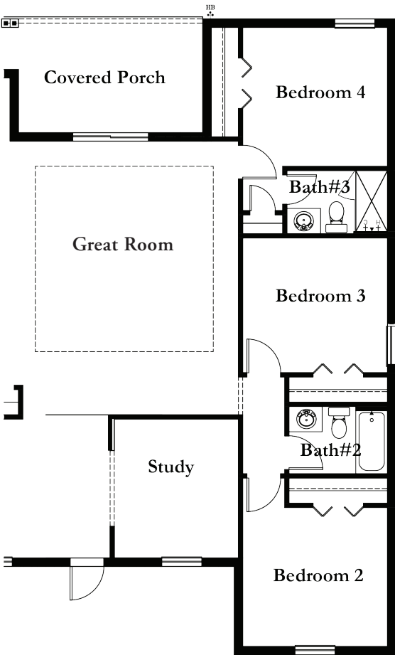
OPTIONAL ENSUITE BATH 3 *ADDS 47 LIVING SQ. FT. *REMOVES 51 SQ. FT. FROM PATIO
